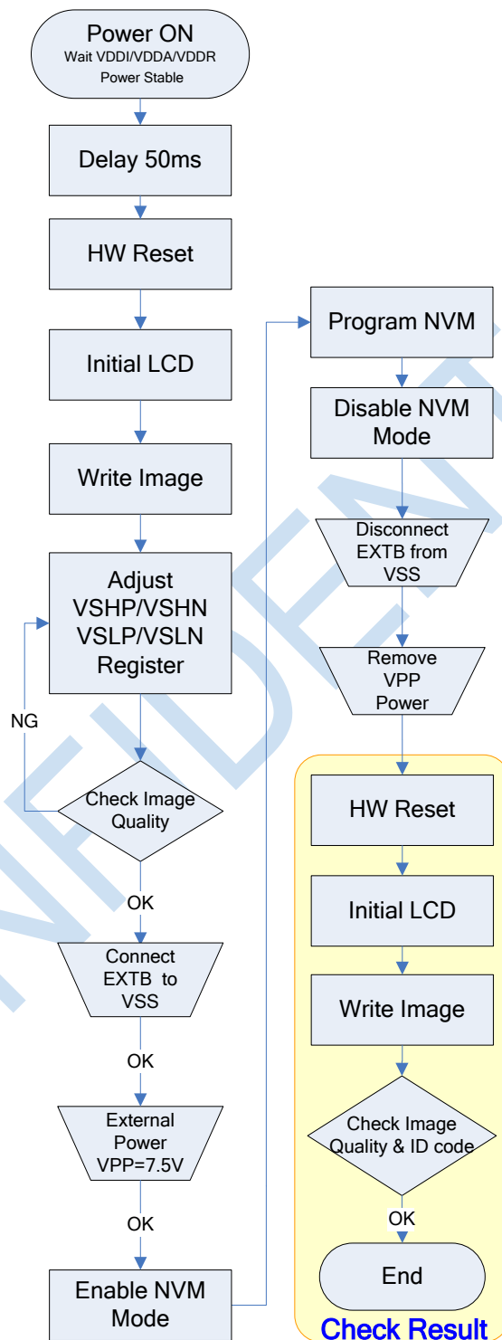
NVM Programming Flow
